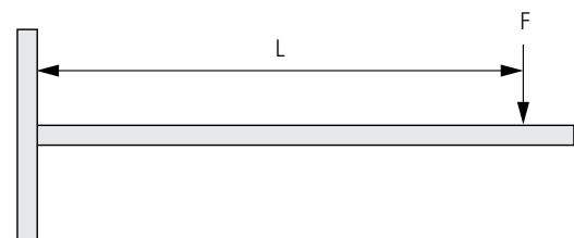
RapidRail® Cantilever Arms One Suspension Point
