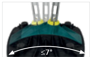
Adjustable to compensate roof pitch up to 7°
