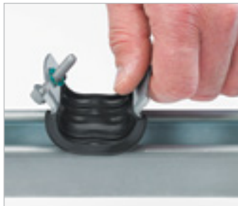
1. Place and turn into strut
