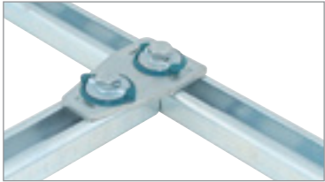
T connector in use with RapidRail®
