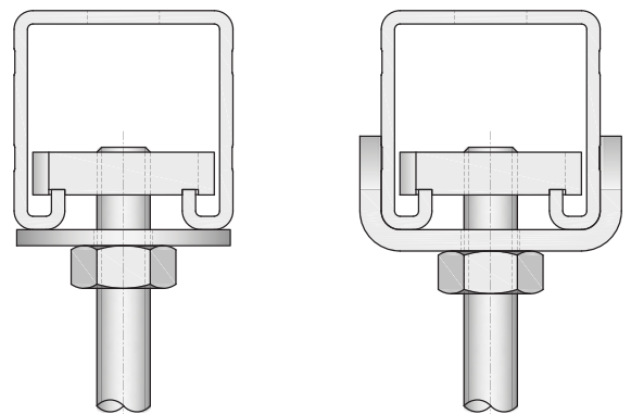
Picture 4: Increase rigidity for loads beneath the channel by using U-shaped washers (right picture) instead of standard flat washers (left picture)
