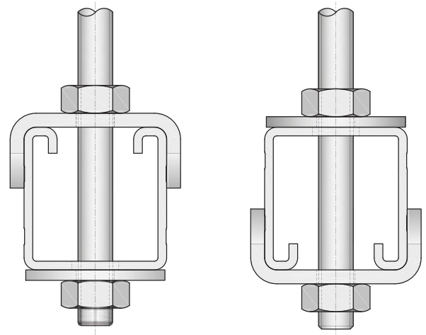
Picture 3: Use of Walraven Strut Washer – U-shaped on the open side of the channel
