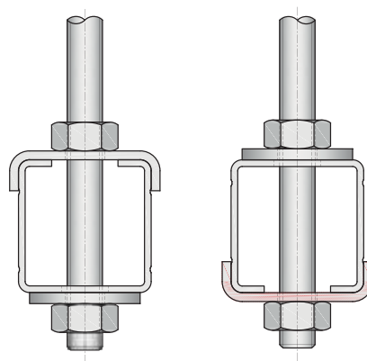
Picture 3: Use of Walraven RapidRail® Washer – U-shaped on the open side of the rail
