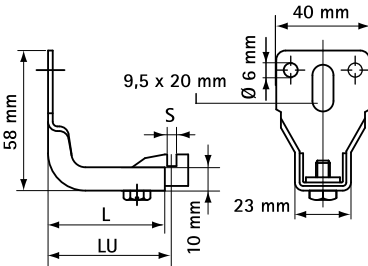
Alternative 0750000 / 0750400 -----BIS-Fixing Set for Isolated Radiator (OS1/ ZVH) 50 mm
